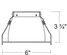
PRLK-400 (4")
