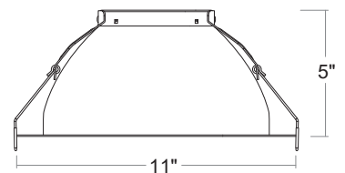
PRLK-1000 (10")
