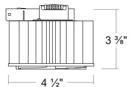
PHSL-1033-5CCT (10")
